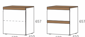
PZ-231 L (1 VRATA / VRATA / DOOR) PZ-231 D (1 VRATA / VRATA / DOOR) PZ-232 (2 PREDALA / LADICE / DRAWERS)
