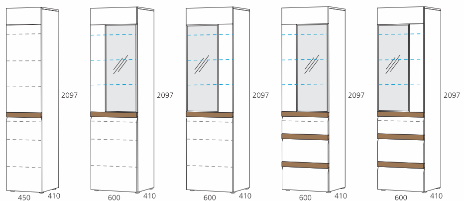
PZ-161 L (1 VRATA / VRATA / DOOR) PZ-161 D (1 VRATA / VRATA / DOOR) PZ-262 L (1 VITRINA / VITRINA / GLASS DOOR) PZ-262 D (1 VITRINA / VITRINA / GLASS DOOR) PZ-263 L (1 VITRINA / VITRINA / GLASS DOOR, 2 PREDALA / LADICE / DRAWERS) PZ-263 D (1 VITRINA / VITRINA / GLASS DOOR, 2 PREDALA / LADICE / DRAWERS)
