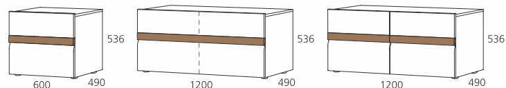
PZ-221G (2 PREDALA / LADICE / DRAWERS) PZ-421G (2 DVOJNA PREDALA / DUPLA LADICE / DOUBLE DRAWERS) PZ-422G (4 PREDALI / LADICE / DRAWERS)
